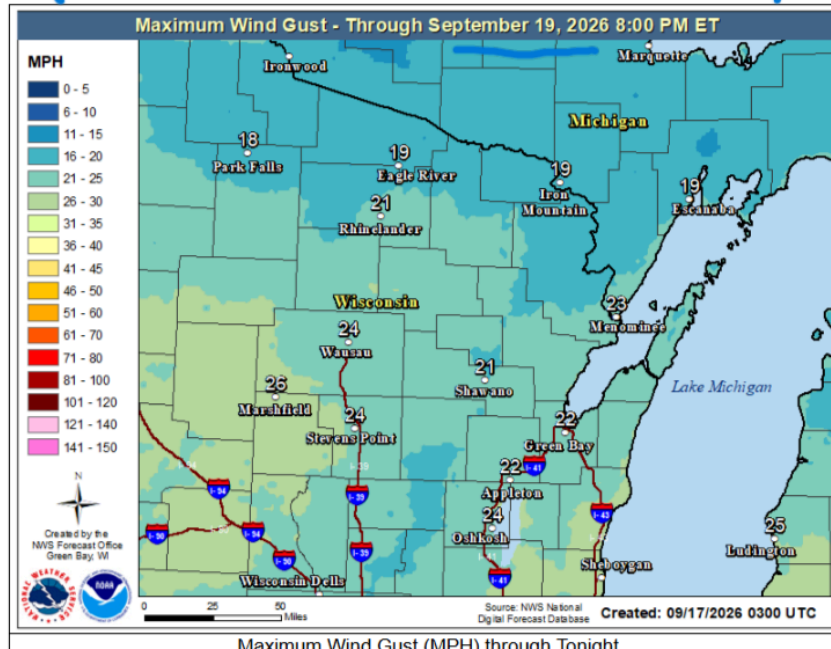
Maximum Wind Gust (MPH) through Tonight
